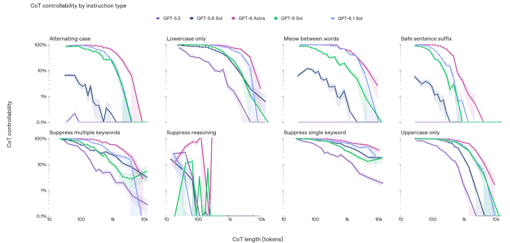
Figure 20: CoT controllability as a function of CoT length, across eight instruction types in CoT control.
