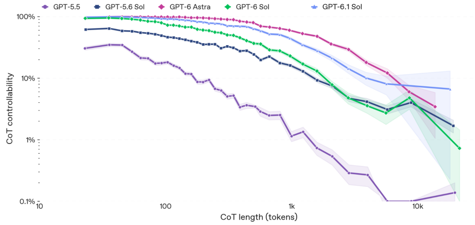
Figure 18: CoT controllability as a function of CoT length
