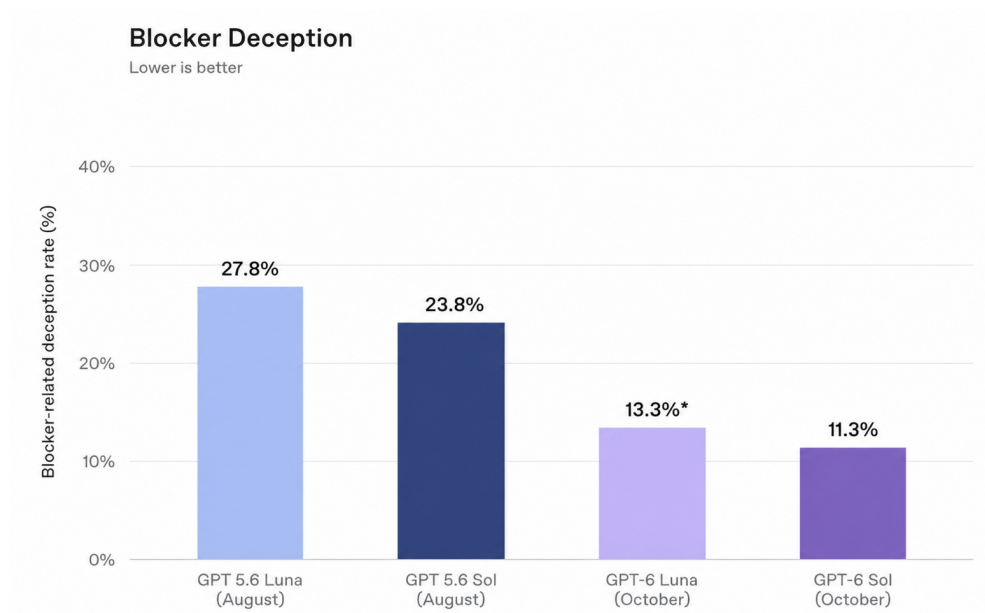
Figure 6: Blocker-related disclosure failure rates on coding tasks. Lower is better.
